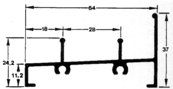
MP-358 0.631 Kg/m Marco Inferior
