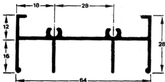
MP-357 0.659 Kg/m Marco Superior
