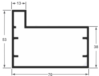
PC-010 (D-141) 1,190 kg/ml
