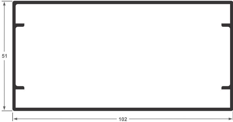
TUB - 4599R 1,833 kg/ml
